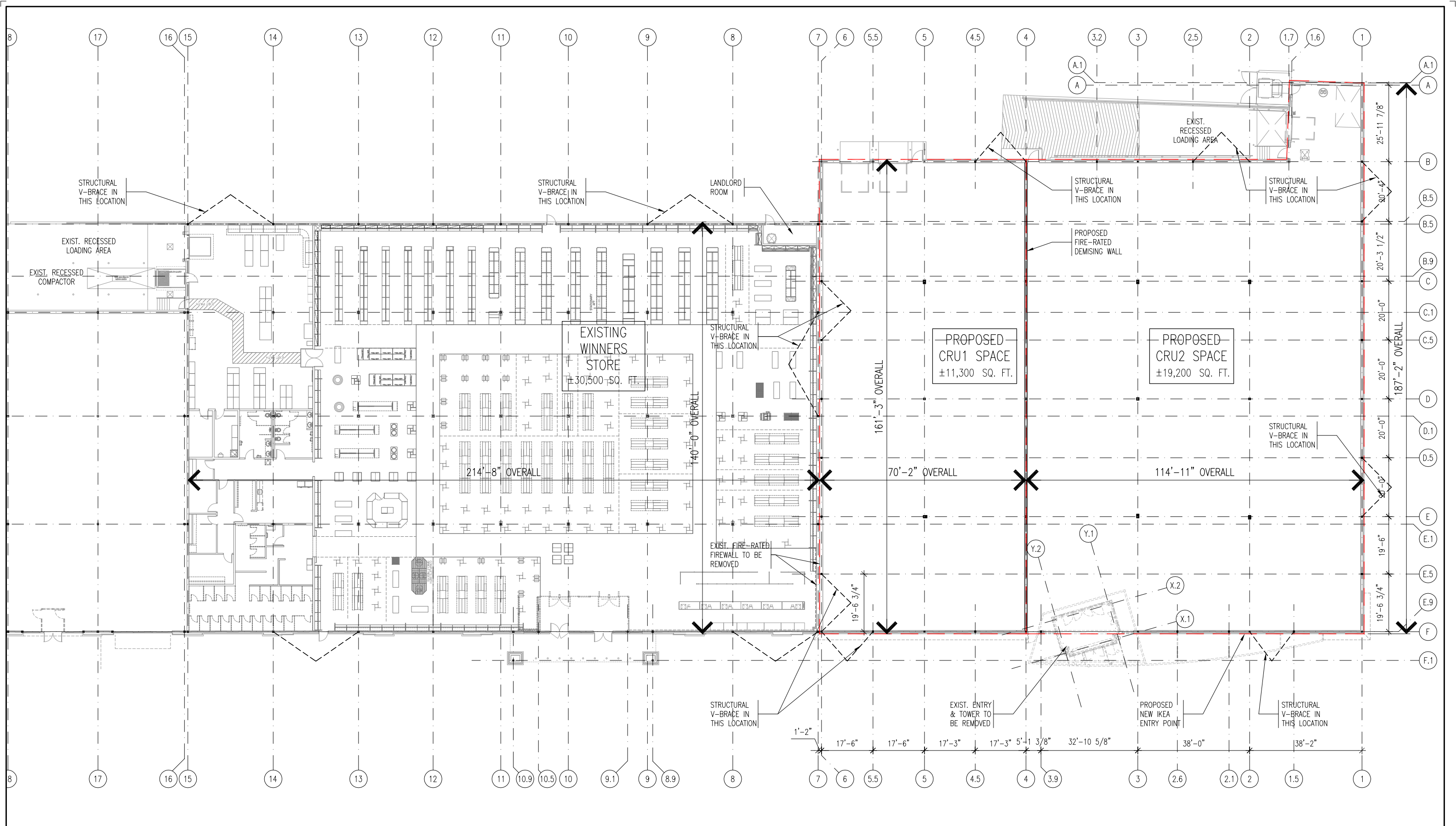
FLOOR PLAN - OPTION#2 SCALE : 1" = 30'-0" 0 5 10 20 30 60 FEET
